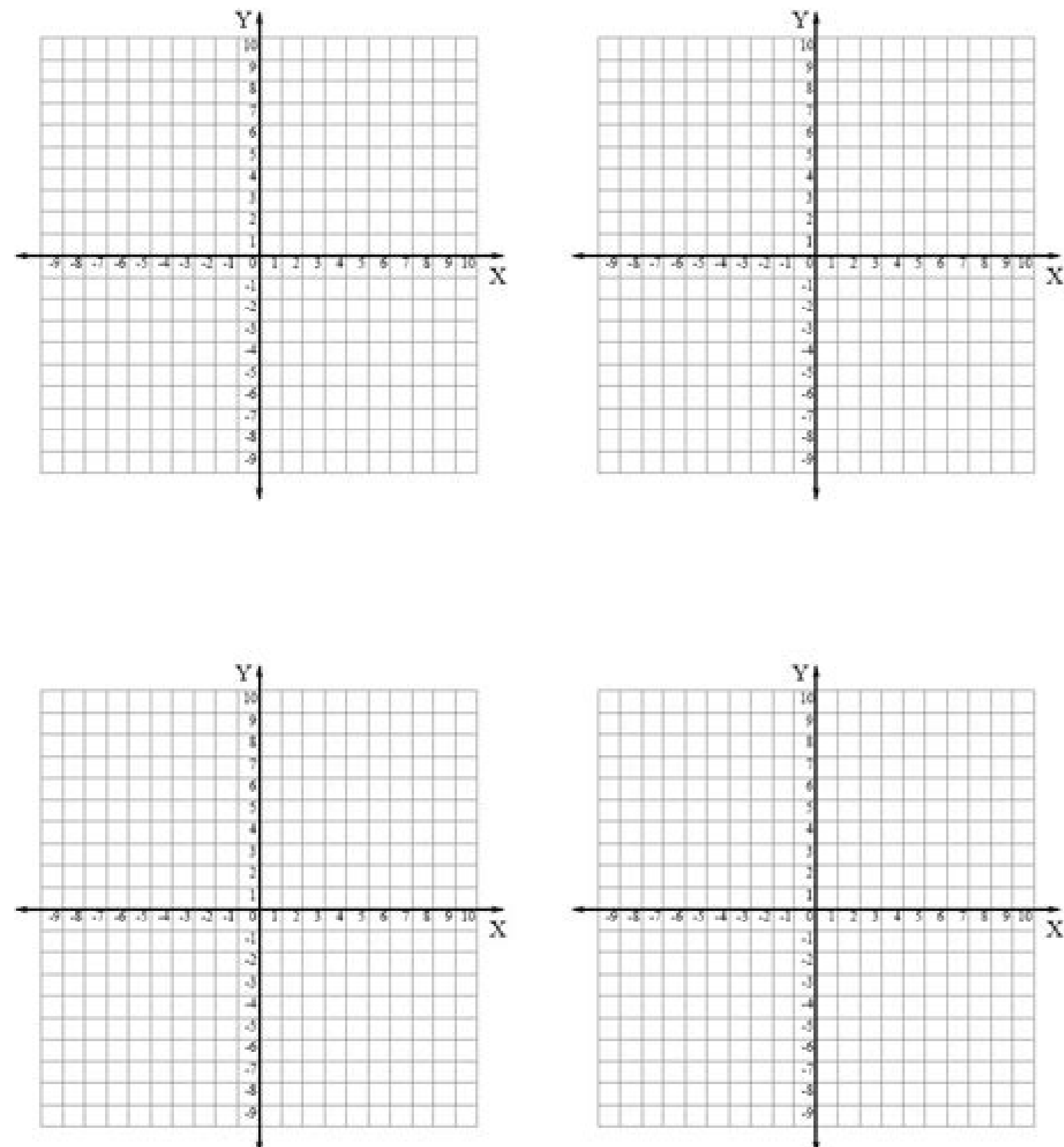
coordinate plane 1
